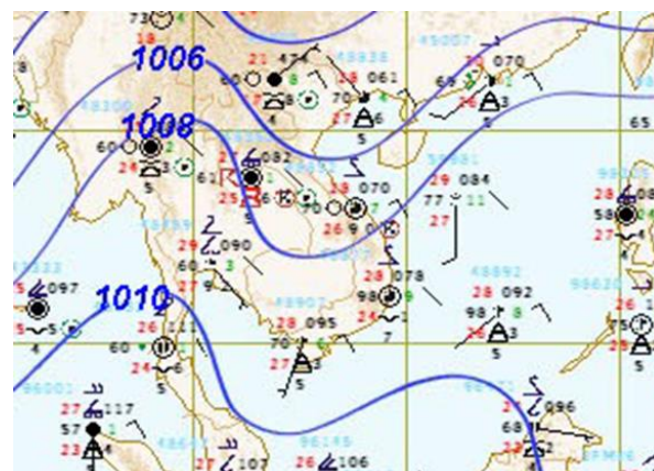
Figure 2: Weather map for 15 th July 2016
