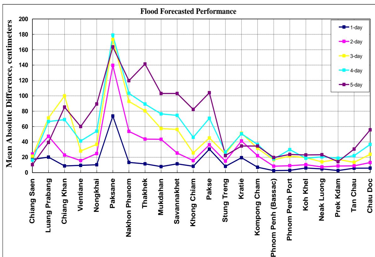
Figure B1: Average flood forecast accuracy along the Mekong mainstream (from 27 th June – 04 th July 2016)
