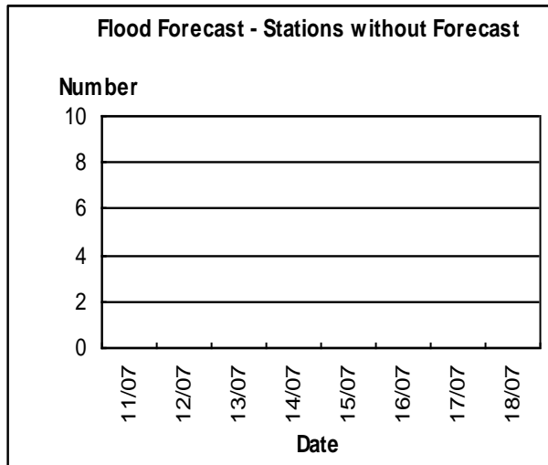
Figure B5: Flood forecast stations without forecast
