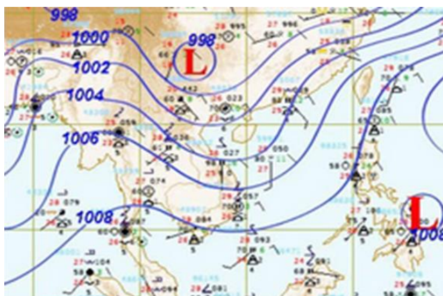
Figure 1: Weather map for 12 nd July 2016
