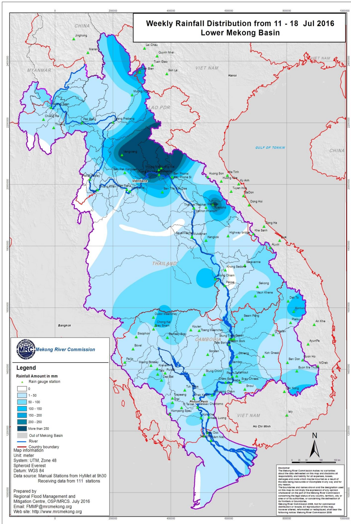
Figure 3: Weekly Rainfall Distribution over the LMB from 11 st – 18 st July, 2016
